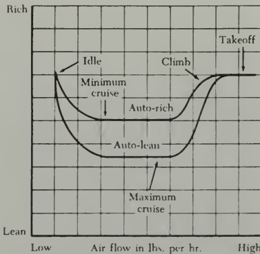
FIGURE 10-37. Typical fuel/air mixture curve for injection-type carburetor.
